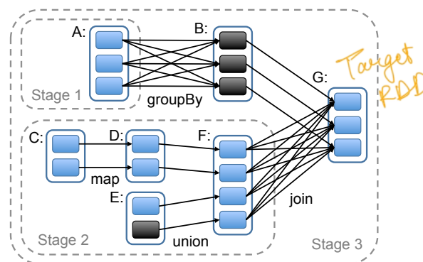
Figure 5: Example of how Spark computes job stages. Boxes with solid outlines are RDDs. Partitions are shaded rectangles, in black if they are already in memory. To run an action on RDD G, we build build stages at wide dependencies and pipeline narrow transformations inside each stage. In this case, stage 1's output RDD is already in RAM, so we run stage 2 and then 3.
