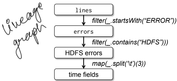
Figure 1: Lineage graph for the third query in our example. Boxes represent RDDs and arrows represent transformations.
